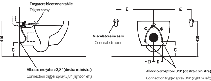
Vaso Sospeso -Wall-hung WC- Hang Wc
