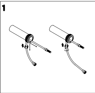
Y1H701 Questo sistema trasforma i WC sospesi e back-to wall in Wc-bidet. This system transforms wall-hung and back-to-wall WC in Wc-bidet.
