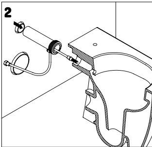
Y1H701 Questo sistema trasforma i WC sospesi e back-to wall in Wc-bidet. This system transforms wall-hung and back-to-wall WC in Wc-bidet.
