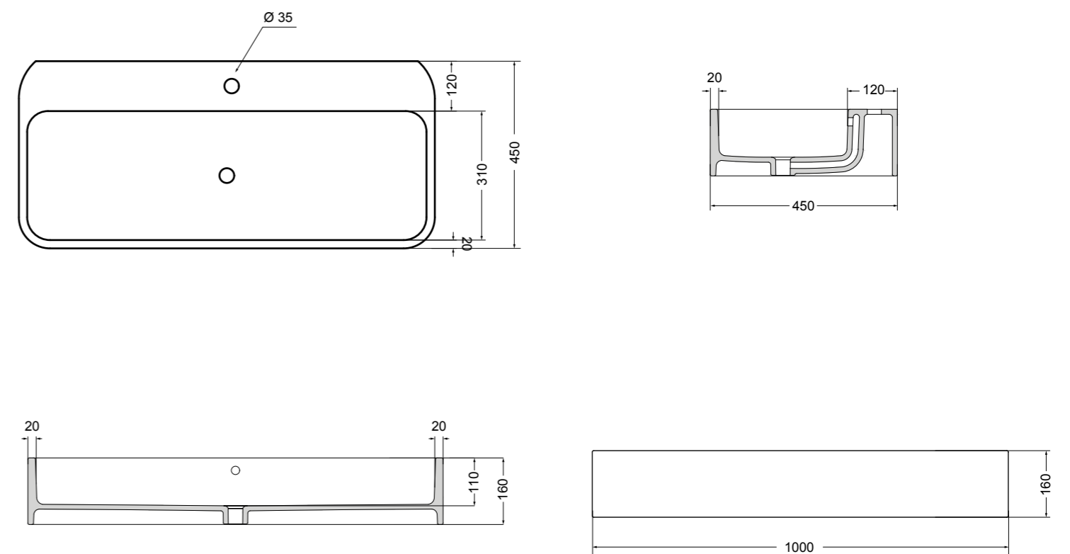
86400 lavabo appoggio/sospeso 100x45 cm_counter-top/wall-hung basin 100x45 cm
